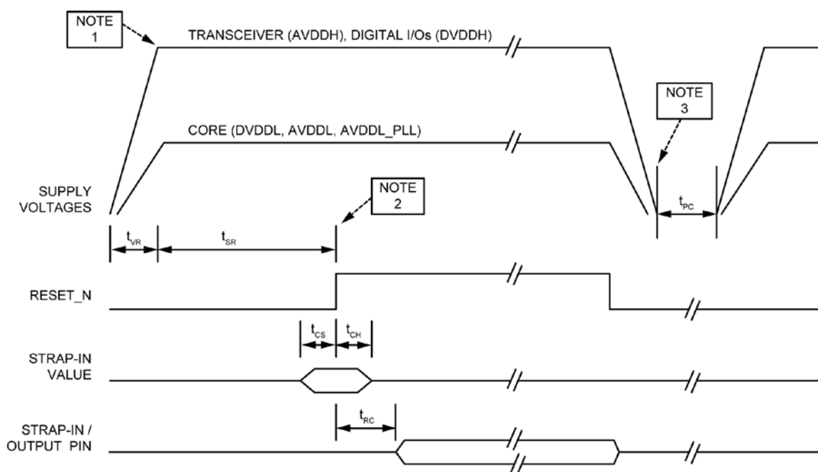
Figure 15. Power-Up/Power-Down/Reset Timing
