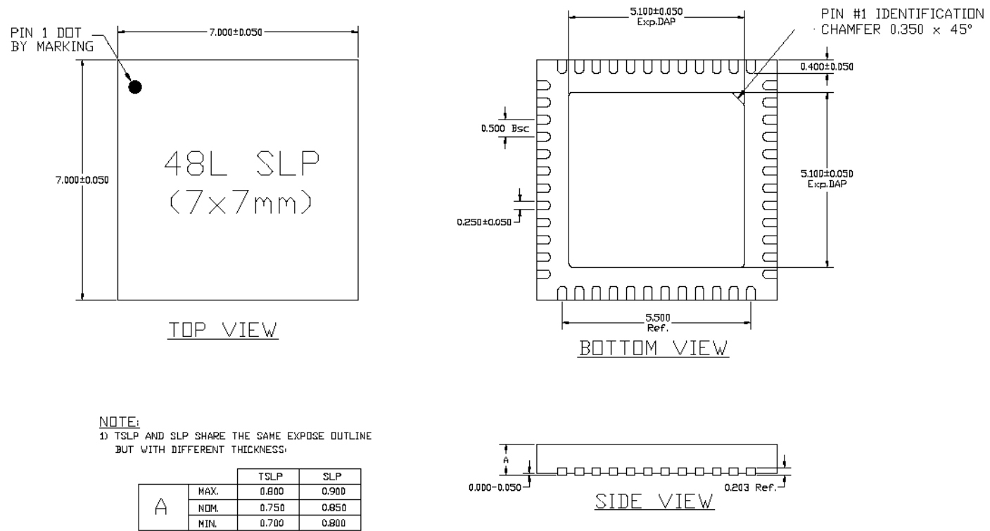
48-Pin (7mm x 7mm) QFN
